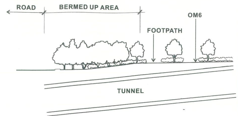
SECTION - B
